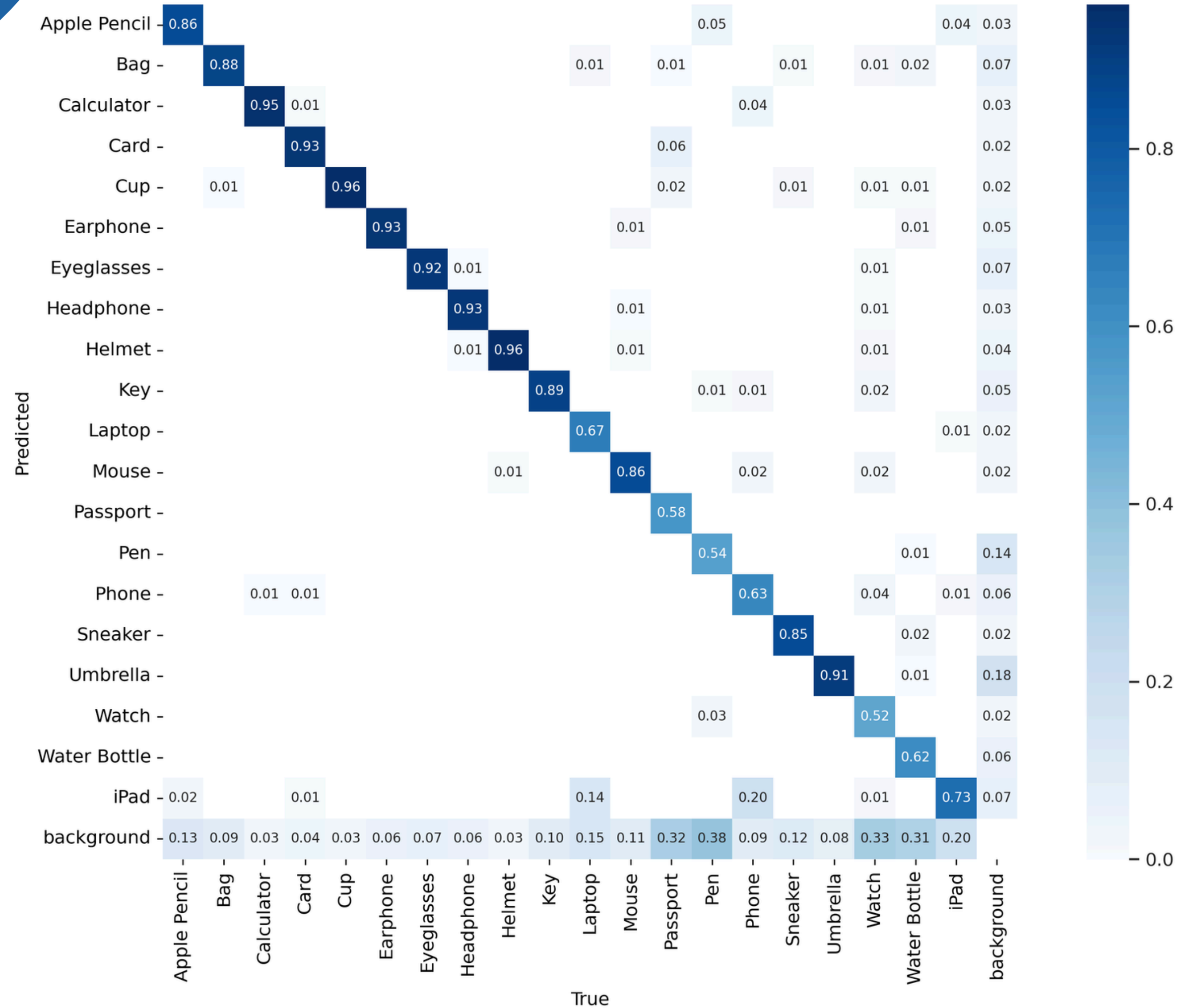
Confusion Matrix
